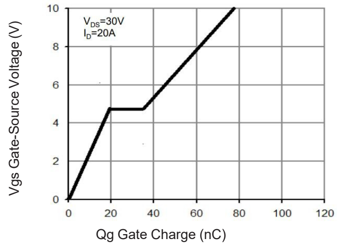
Figure 5 Gate Charge
