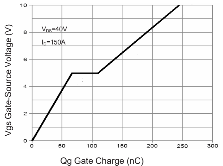
Figure 5 Gate Charge
