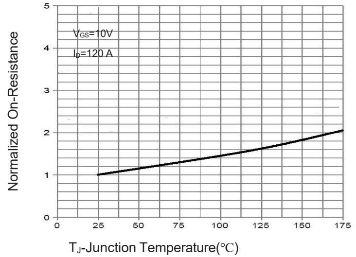
Figure 4 Rdson-Junction Temperature
