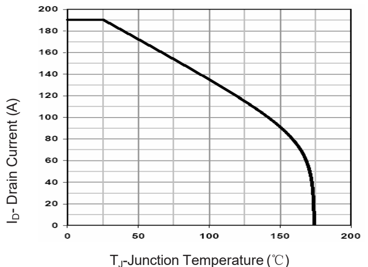
Figure 10 Current De-rating
