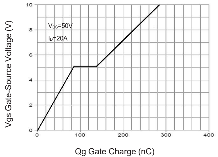
Figure 5 Gate Charge
