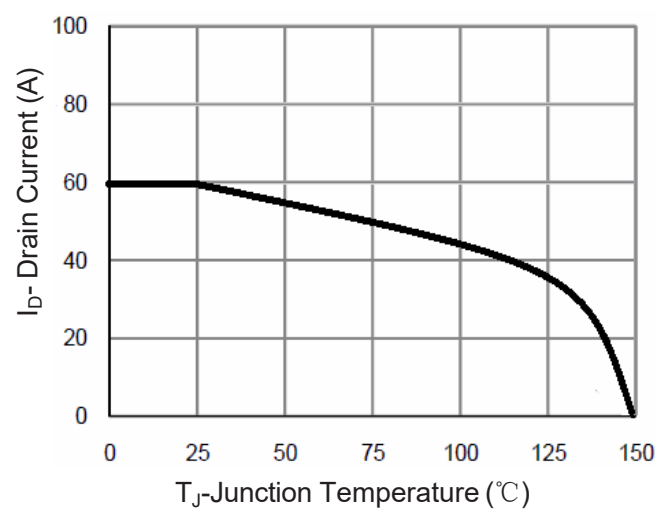
Figure 10 Current De-rating
