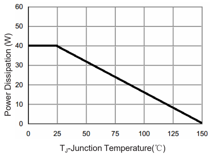
Figure 9 Power De-rating
