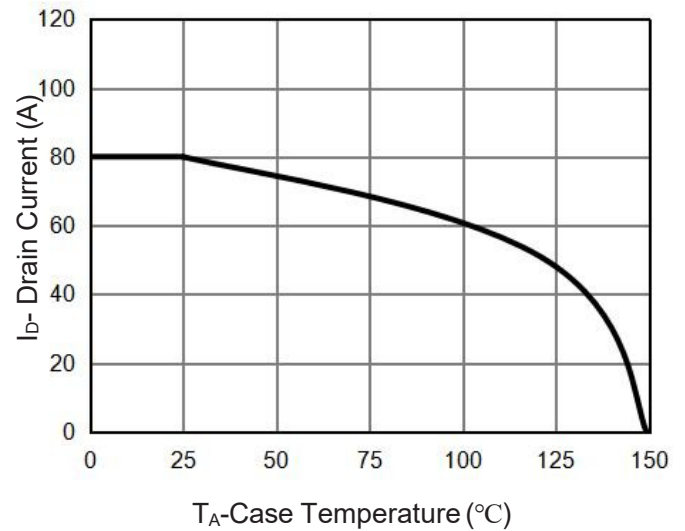
Figure 10 Current De-rating
