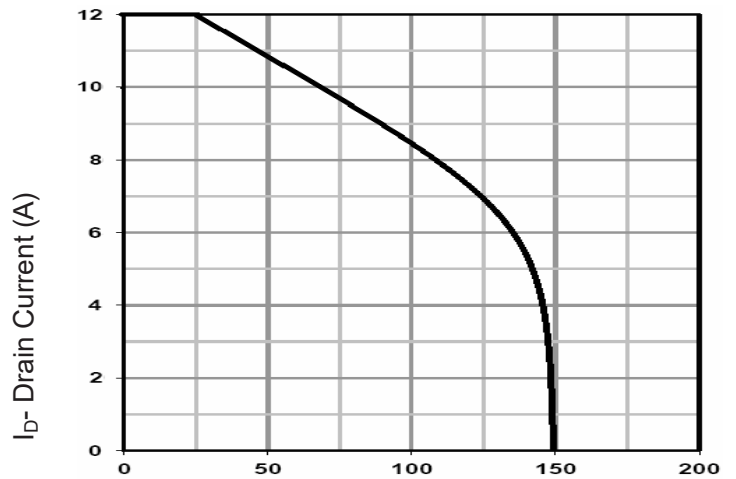
TJ-Junction Temperature (°C) Figure 10 Current De-rating
