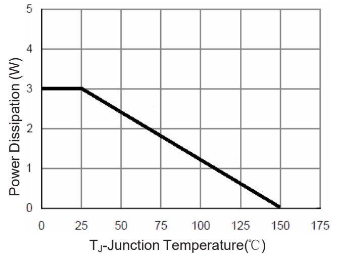
Figure 10 Power De-rating
