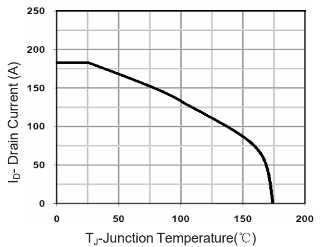
Figure 10 Current De-rating
