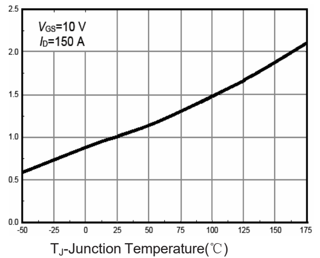
Figure 4 Rdson-Junction Temperature
