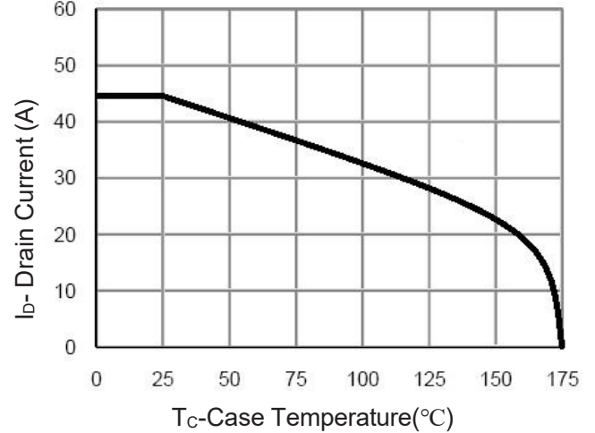
Figure 10 Current De-rating
