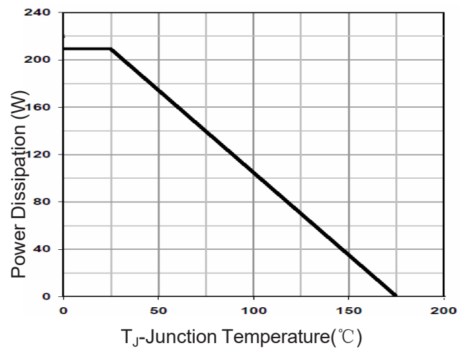
Figure 9 Power De-rating
