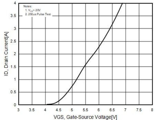
Figure4. Transfer characteristics
