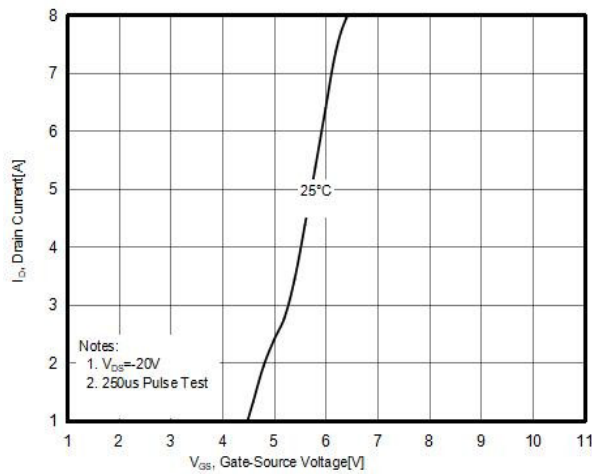
Figure3. Transfer characteristics
