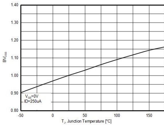
Figure7. BV_{DS} vs Junction Temperature
