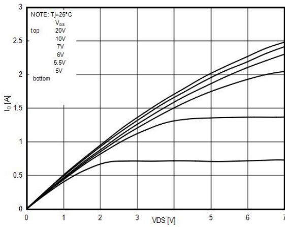
Figure3. Output characteristics
