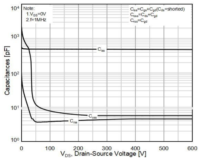
Figure10. Capacitance
