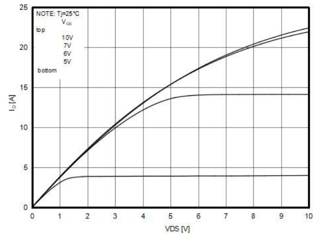
Figure4. Output characteristics
