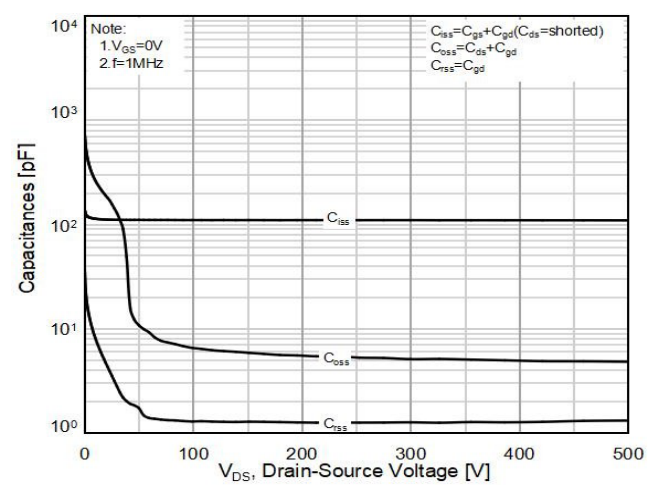
Figure10. Capacitance
