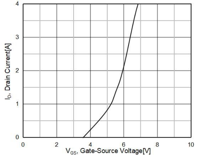
Figure4. Transfer characteristics
