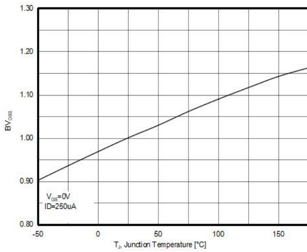
Figure7. BV_{DS} vs Junction Temperature
