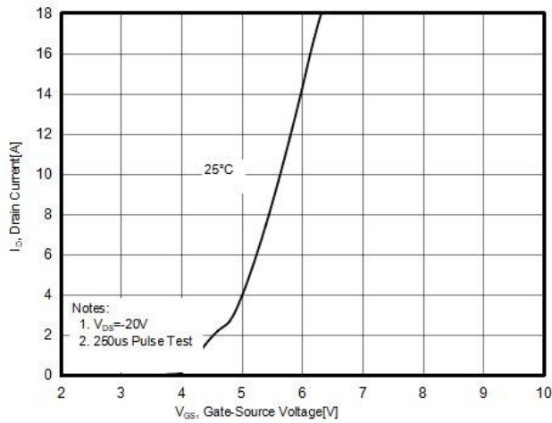
Figure3. Transfer characteristics
