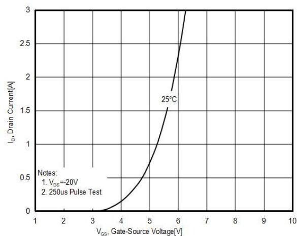
Figure4. Transfer characteristics
