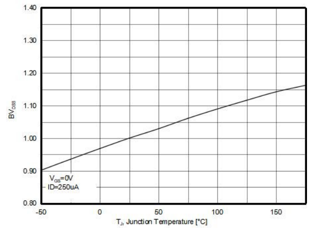
Figure4. BV_{DSS} vs Junction Temperature
