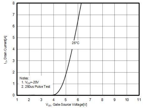
Figure10. Transfer characteristics
