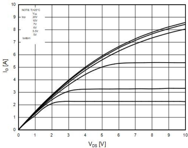
Figure3. Output characteristics
