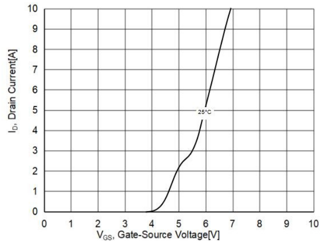
Figure4. Transfer characteristics
