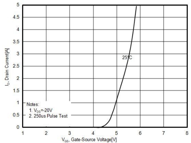
Figure4. Transfer characteristics
