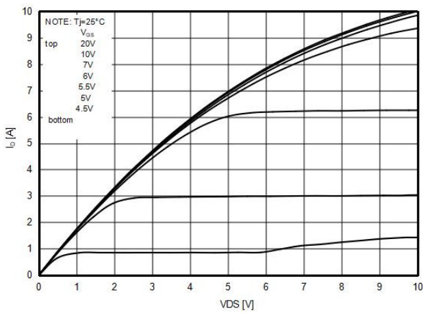
Figure3. Output characteristics
