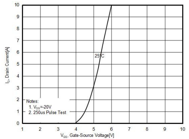
Figure4. Transfer characteristics
