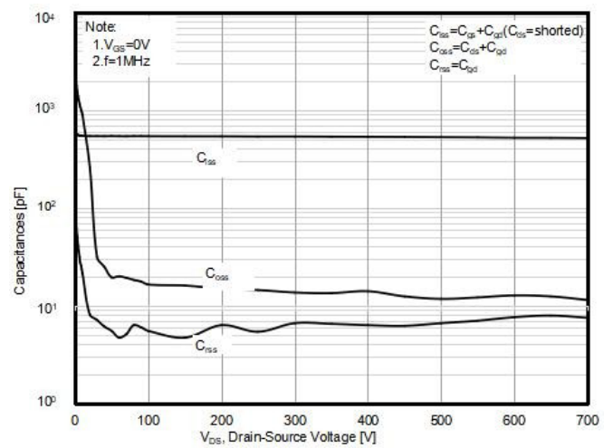
Figure10. Capacitance
