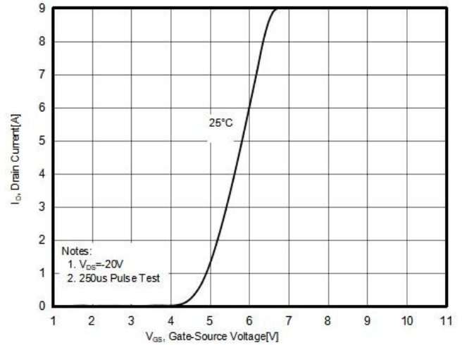
Figure4. Transfer characteristics
