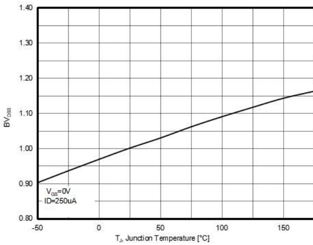
Figure7. BV_{DS} vs Junction Temperature
