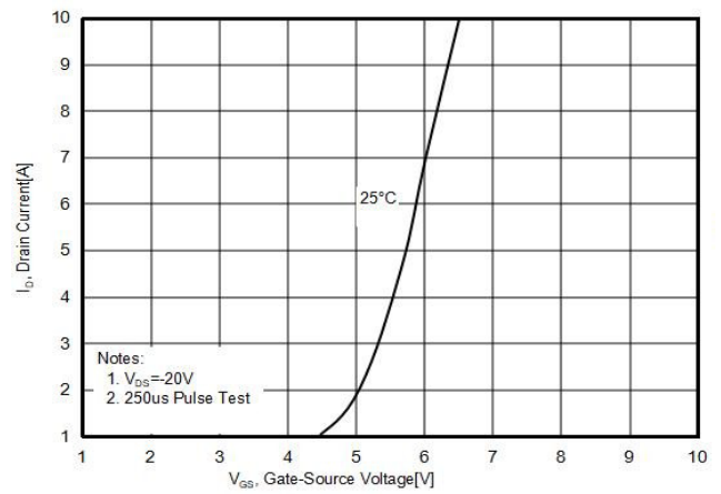
Figure4. Transfer characteristics
