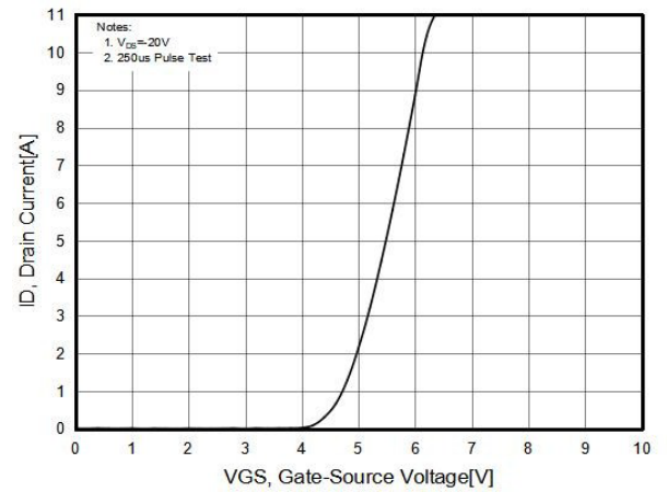
Figure8. Transfer characteristics
