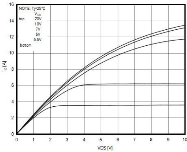
Figure3. Output characteristics
