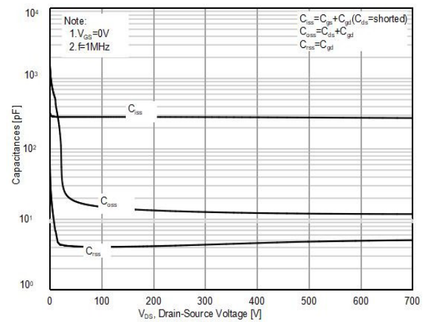
Figure10. Capacitance
