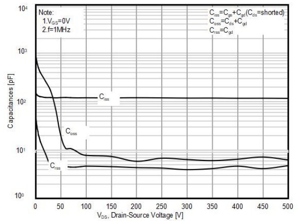
Figure10. Capacitance
