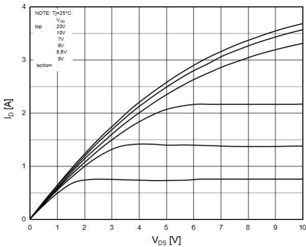
Figure3. Output characteristics
