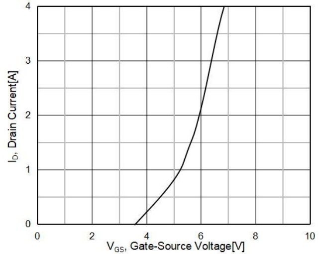
Figure4. Transfer characteristics
