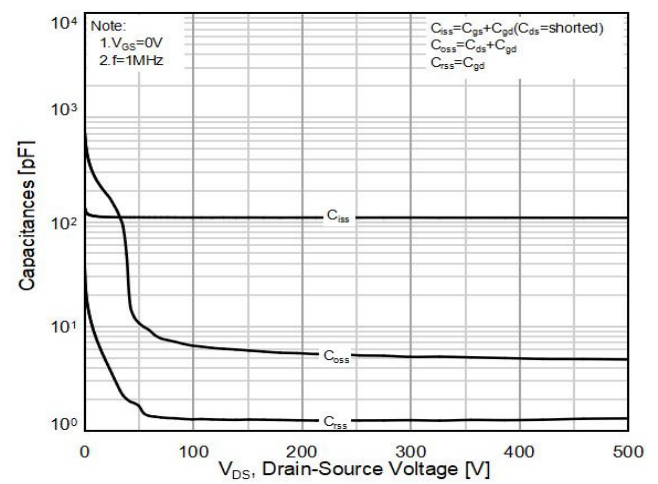
Figure10. Capacitance
