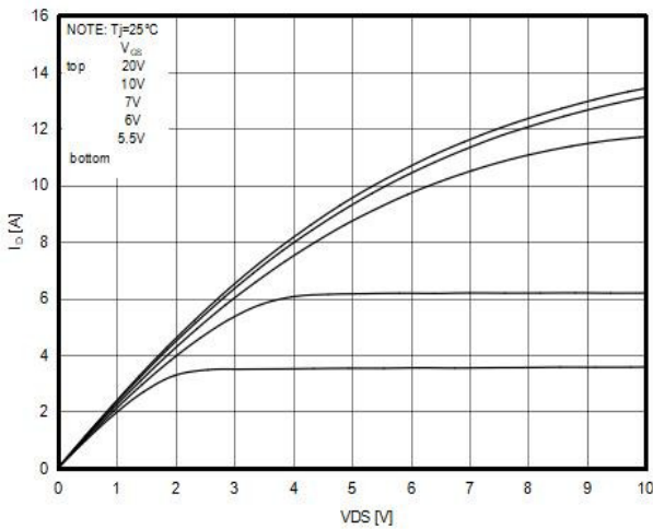
Figure3. Output characteristics
