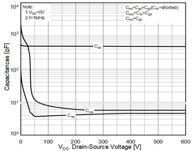
Figure10. Capacitance
