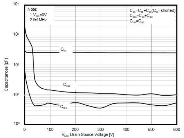
Figure2. Capacitance
