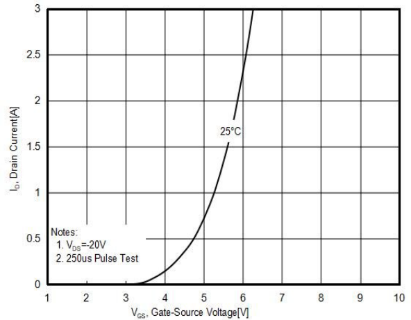
Figure4. Transfer characteristics
