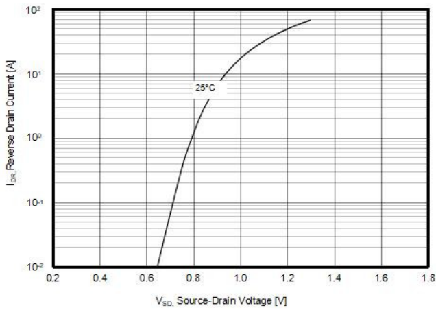
Figure9. Source-Drain Diode Forward Voltage
