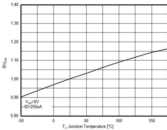
Figure7. BV_{DS} vs Junction Temperature
