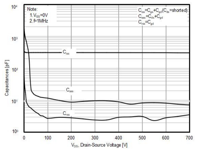
Figure10. Capacitance
