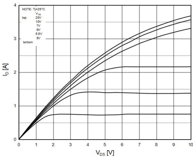
Figure3. Output characteristics
