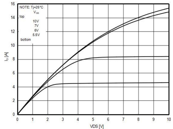
Figure4. Output characteristics
