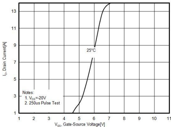
Figure3. Transfer characteristics
