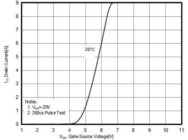
Figure4. Transfer characteristics
