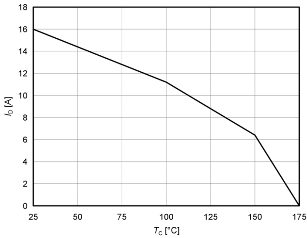
Figure7. Maximum I_D vs Junction Temperature
