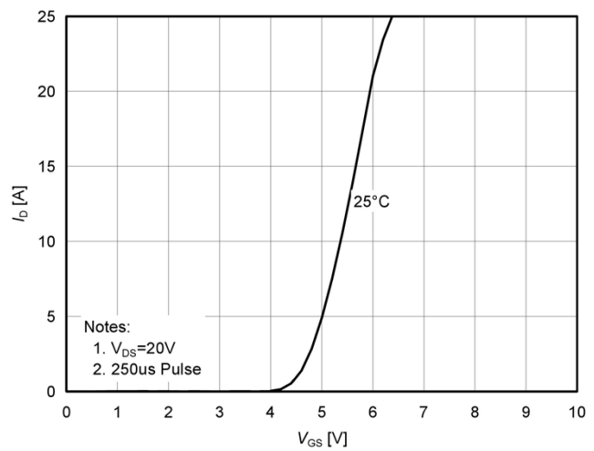
Figure10. Transfer characteristics
