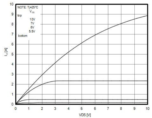
Figure4. Output characteristics
