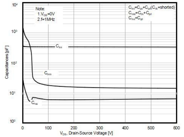
Figure2. Capacitance
