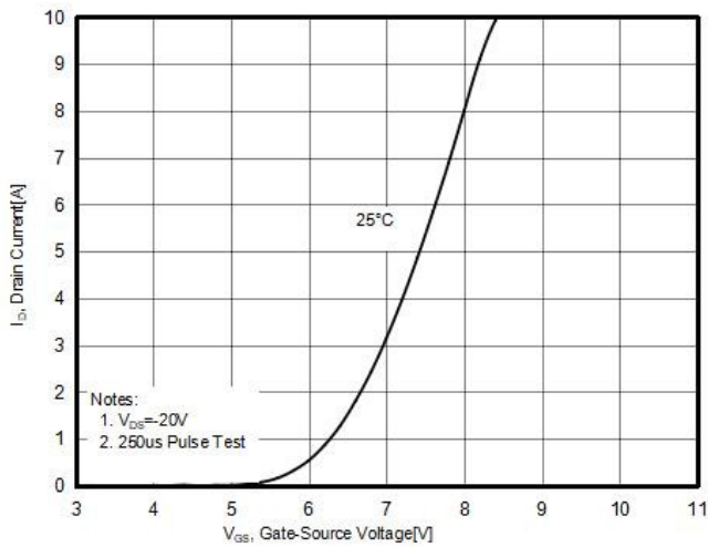
Figure1. Transfer characteristics
