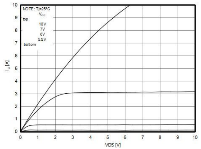
Figure2. Output characteristics
