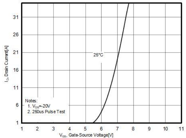
Figure6. Transfer characteristics
